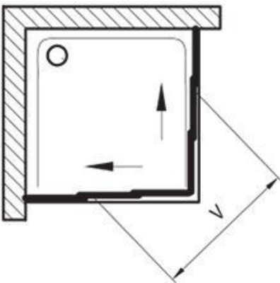
ASRV3 + ASRV3
