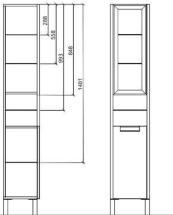
Bokorys
